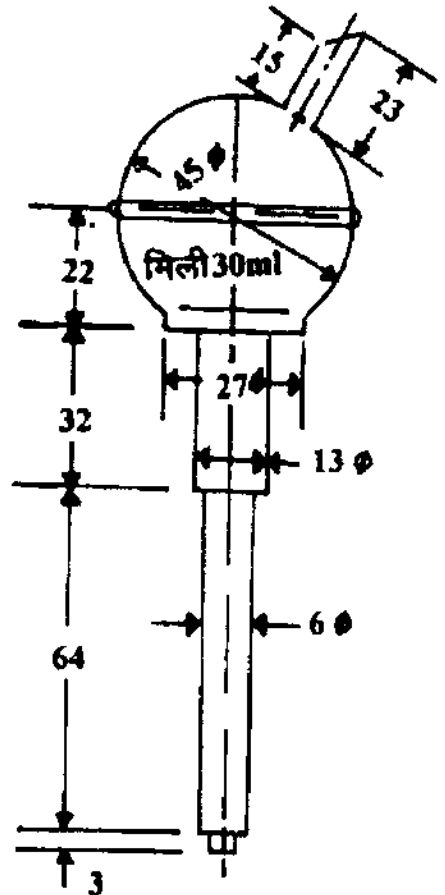
SHAPE AND NOMINAL DIMENSIONS OF AUTOMATIC LIQUOR MEASURE
